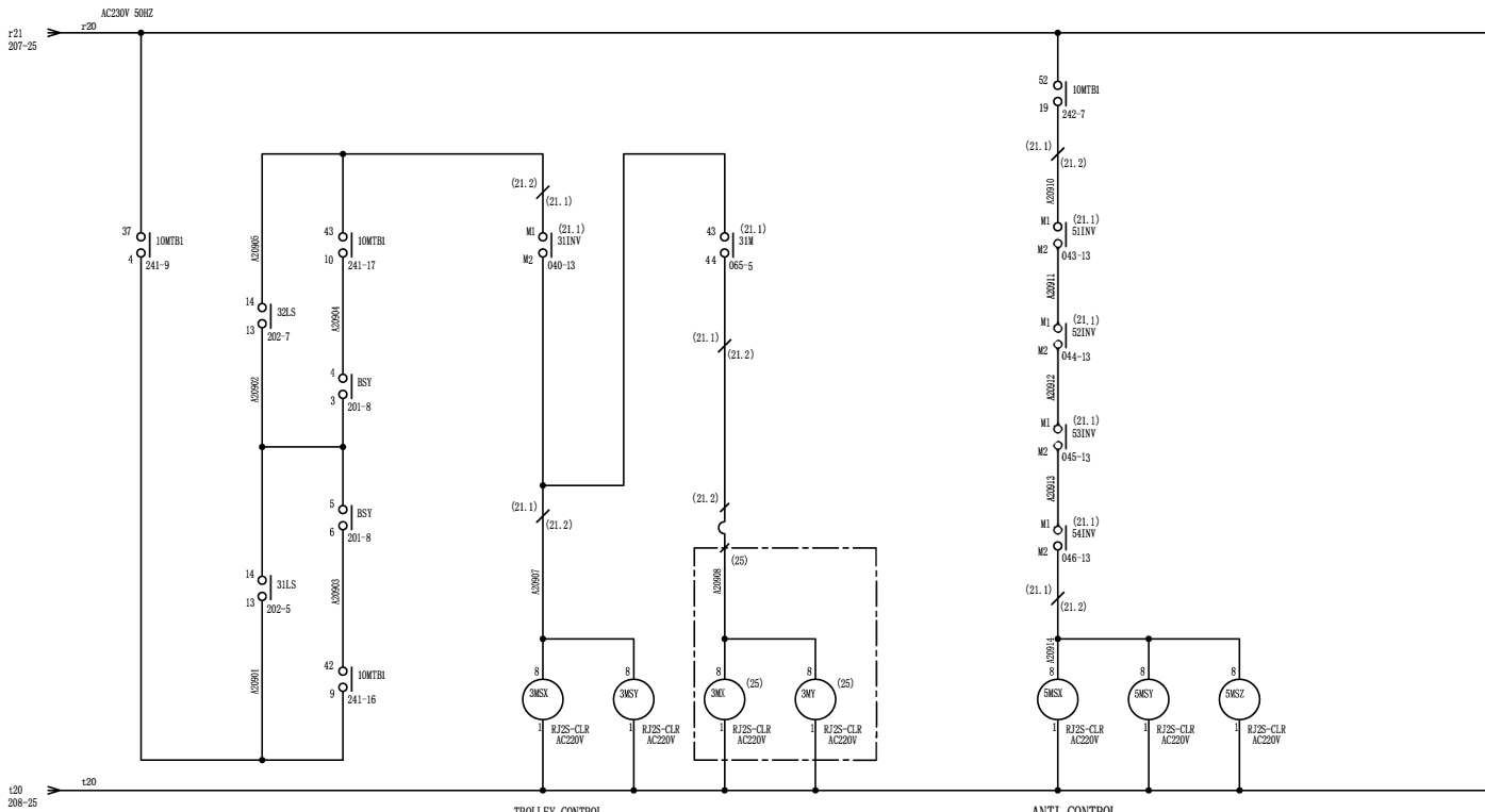
TROLLEY CONTROL
